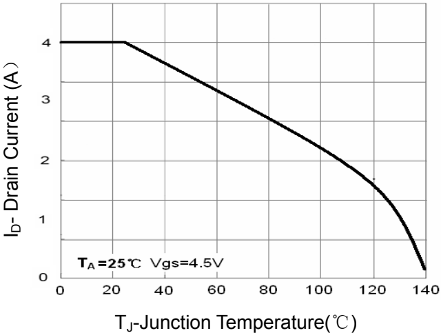
Figure 4 Drain Current
